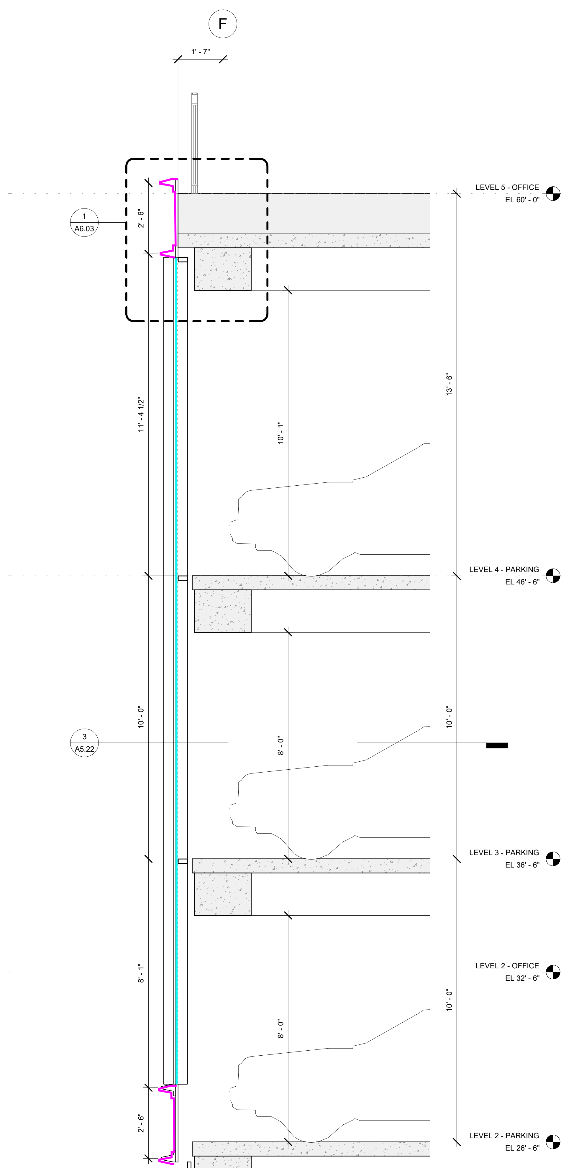
2 SECTION 1/2" = 1'-0"
