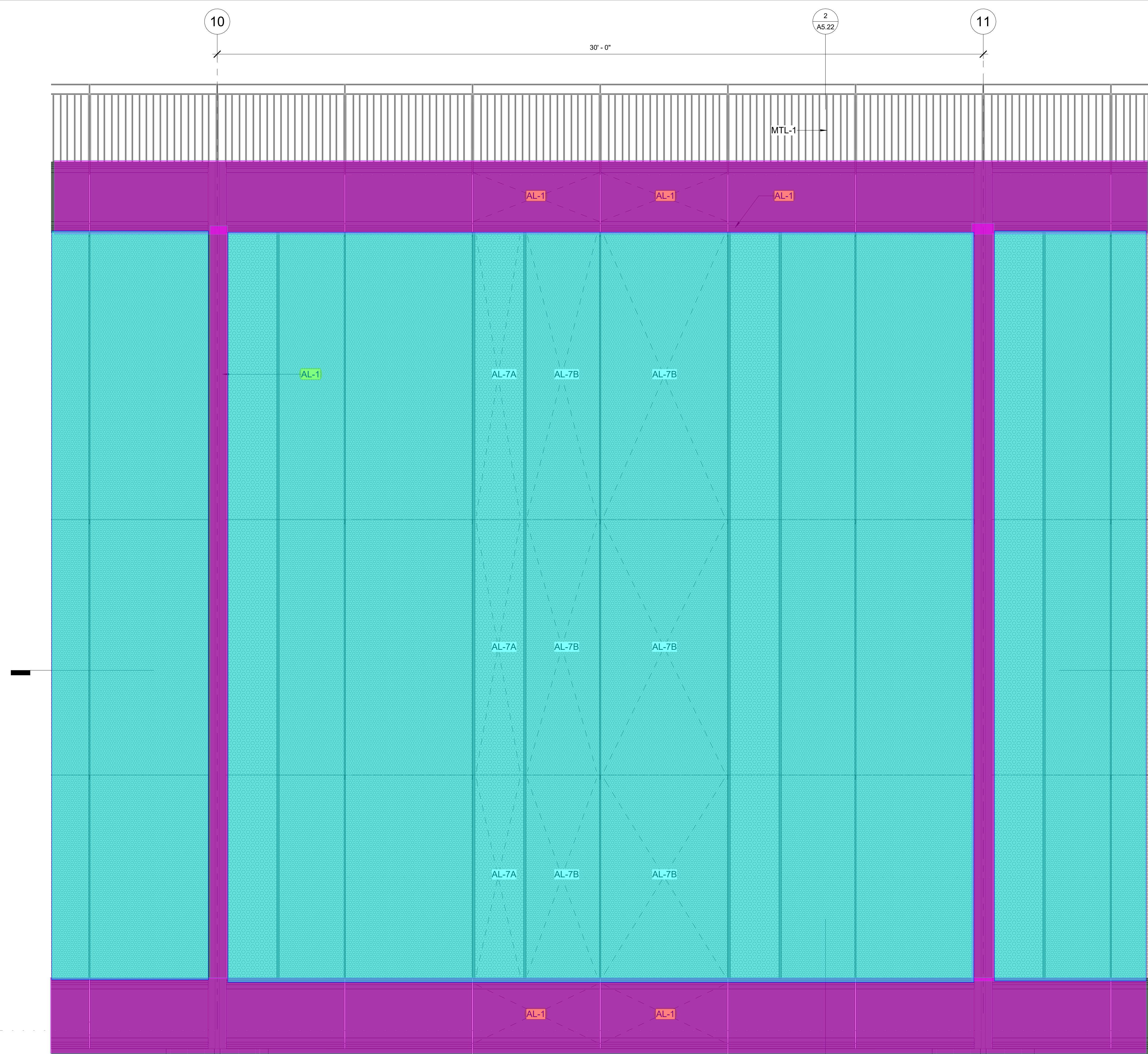
1 ELEVATION 1/2" = 1'-0"
